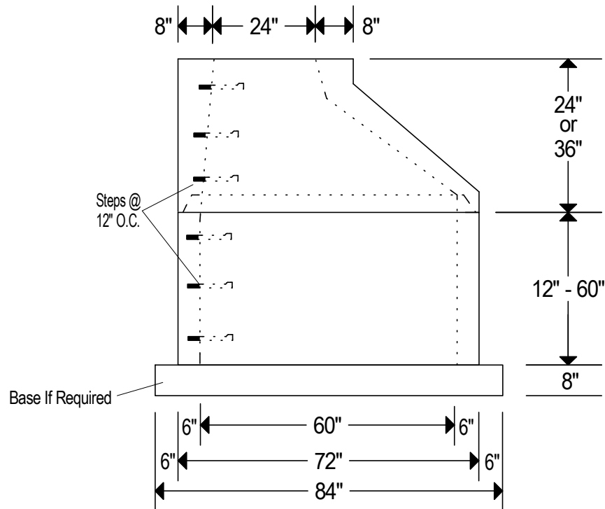
60" x 13" Insert Cover With 24" Opening
