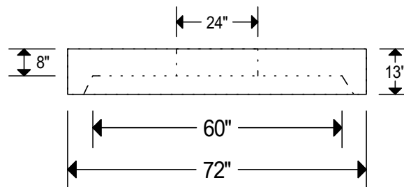
60" x 13" Insert Cover With 24" Opening
