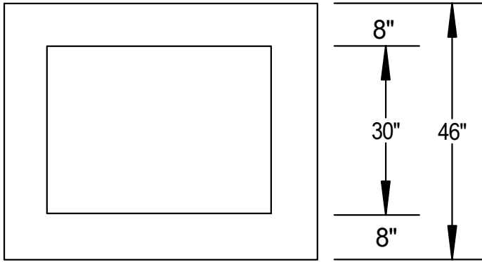
Section Of End View Shown With Adjustable Curb Box.
