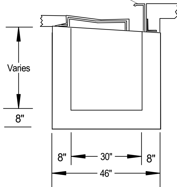
Section Of End View Shown With Adjustable Curb Box.
